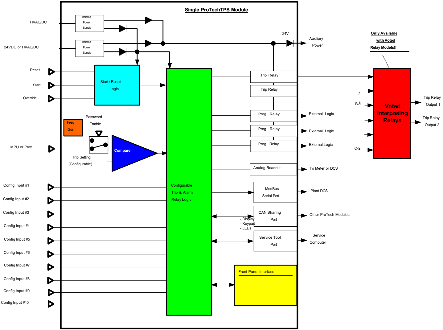
Single Module Functional Diagram
