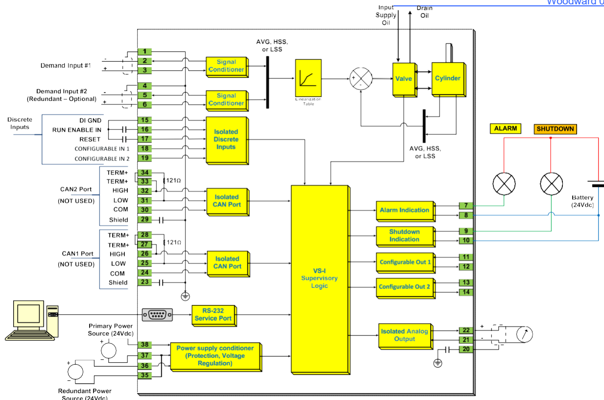
Figure 6. VariStroke-GI Interface
