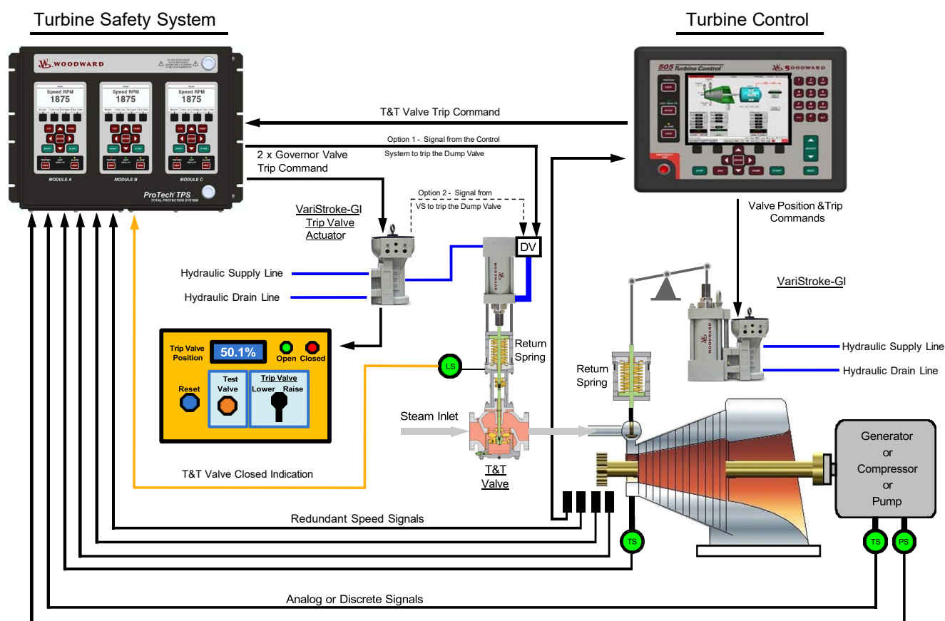
Figure 3. Typical VariStroke-GI Applications
