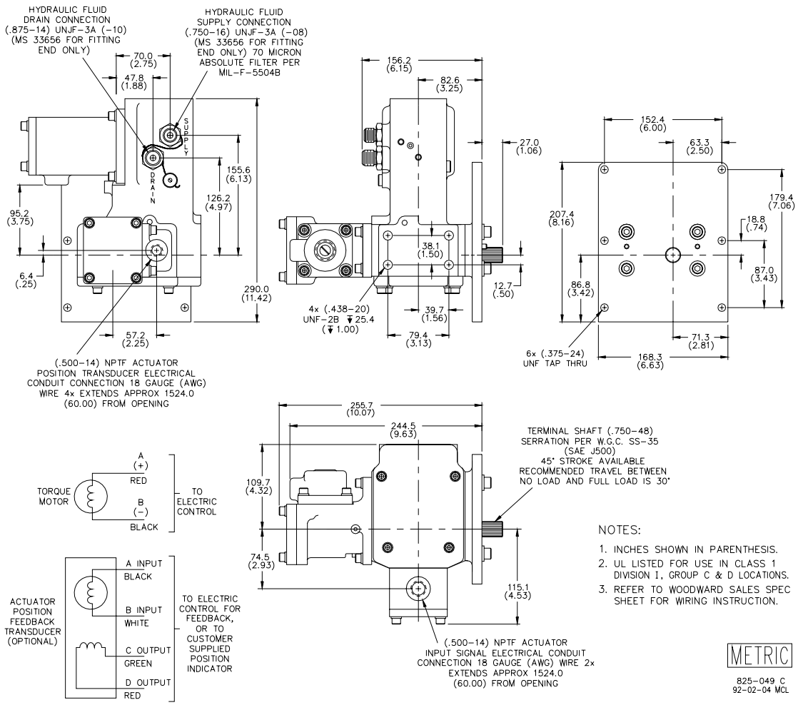
Single Coil TM-55P Actuator Outline Drawing (Do not use for construction)
