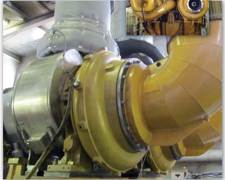
After: Napier NA297 turbocharger installed with new platform and air intake.
